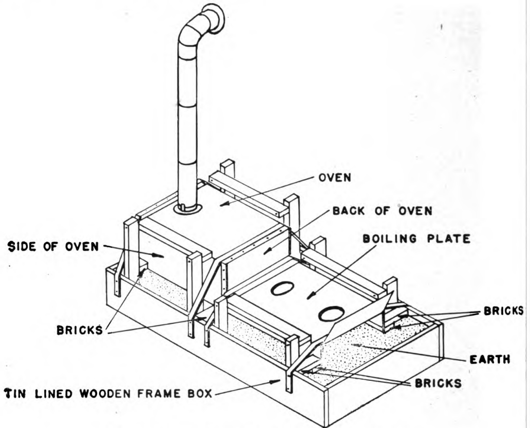
FIGURE 39.—Field range No. 1 installed in baggage car.
